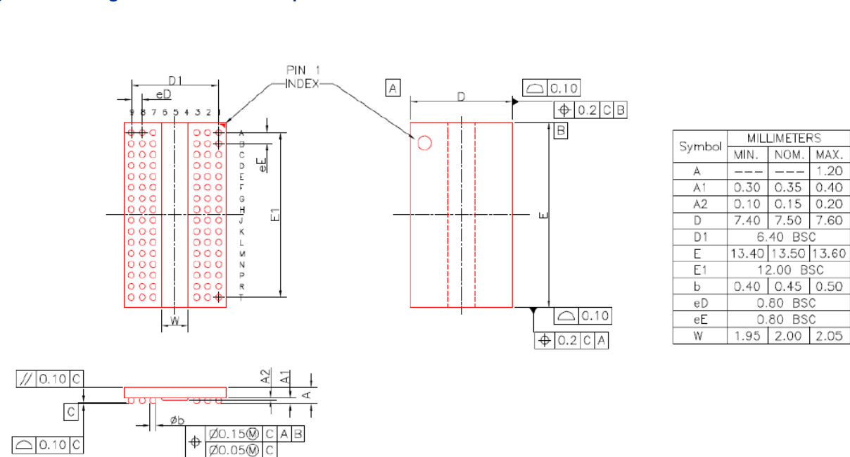
Figure 7 - Package outline for x16 Component
