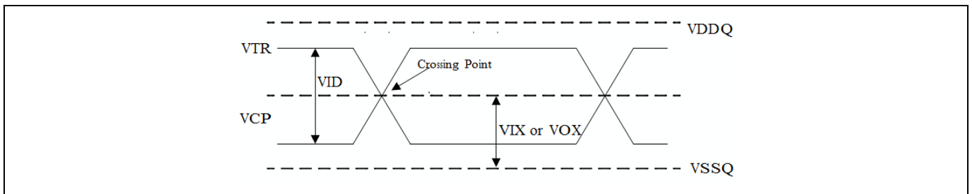
Figure 4 - Differential DC and AC Input and Output Logic Levels Diagram
