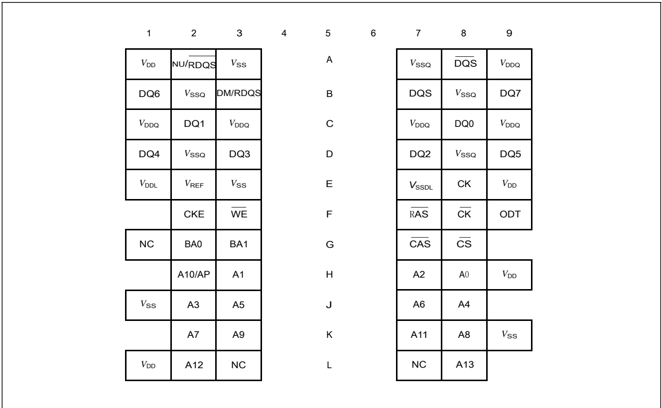
Figure 1 - Chip Configuration for x8 Components, TFBGA-60 (Top view)
