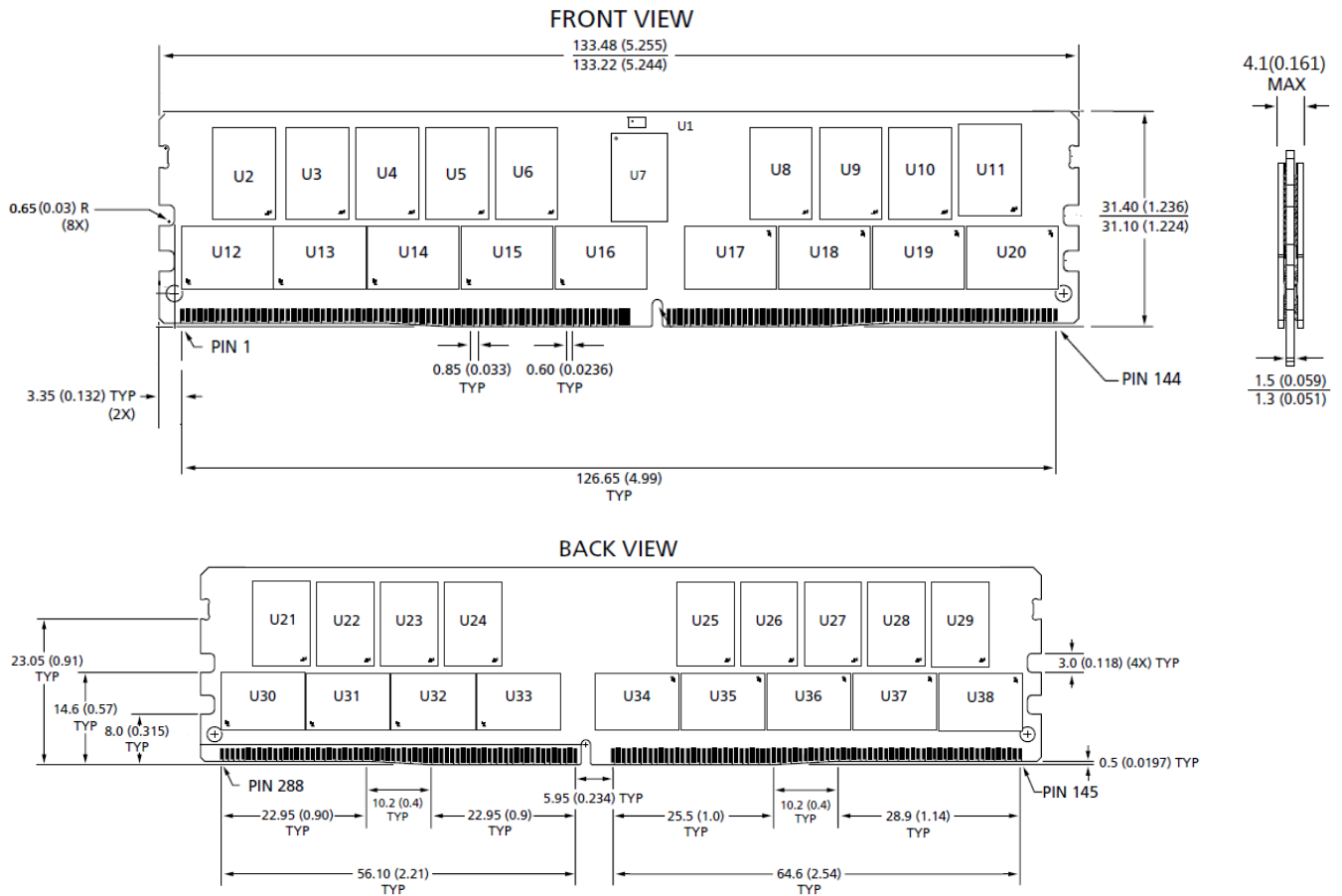
Figure 4 - Package Dimensions_SCQ32GP12H1F1C-26V
