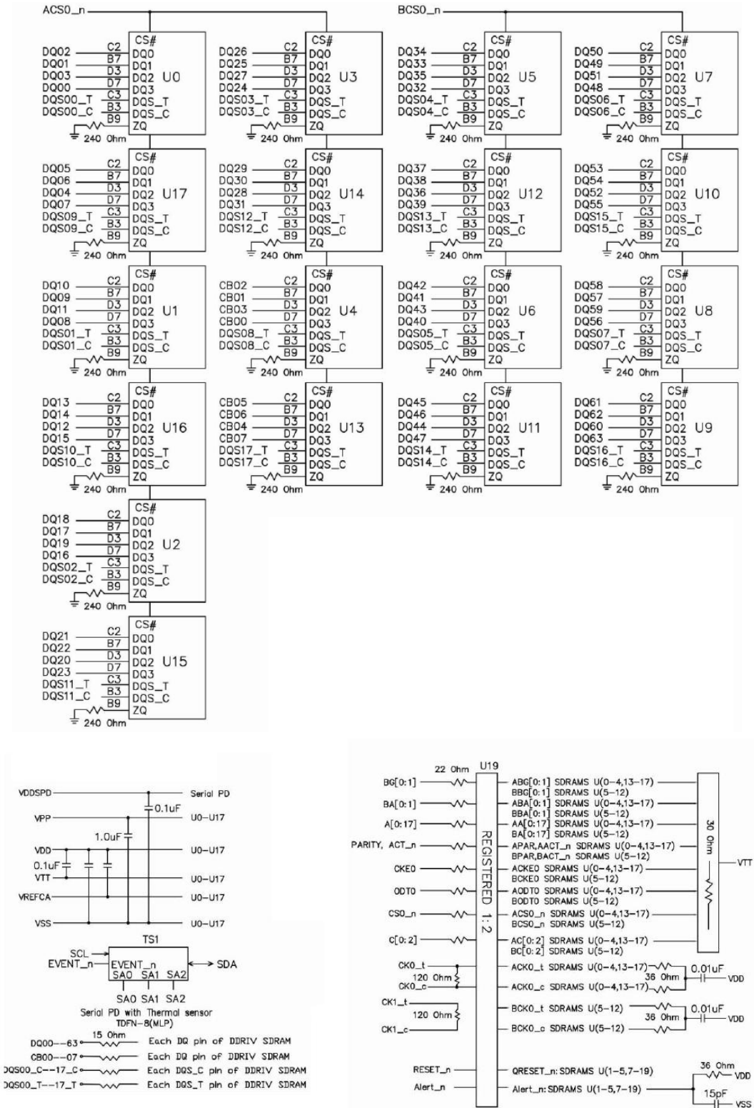
Figure 1 - Function Block Diagram_SCQ16GP02H1F1C-26V
