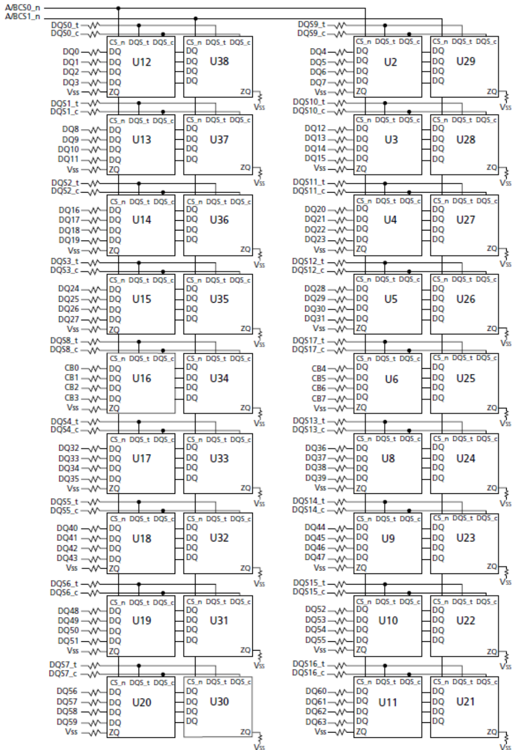
Figure 2 - Function Block Diagram_SCQ32GP12H1F1C-26V
