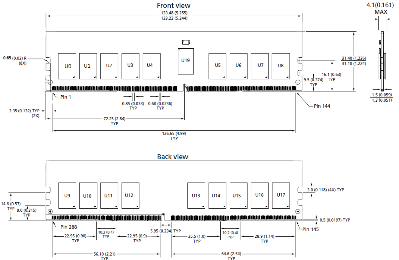
Figure 3 - Package Dimensions_SCQ16GP02H1F1C-26V
