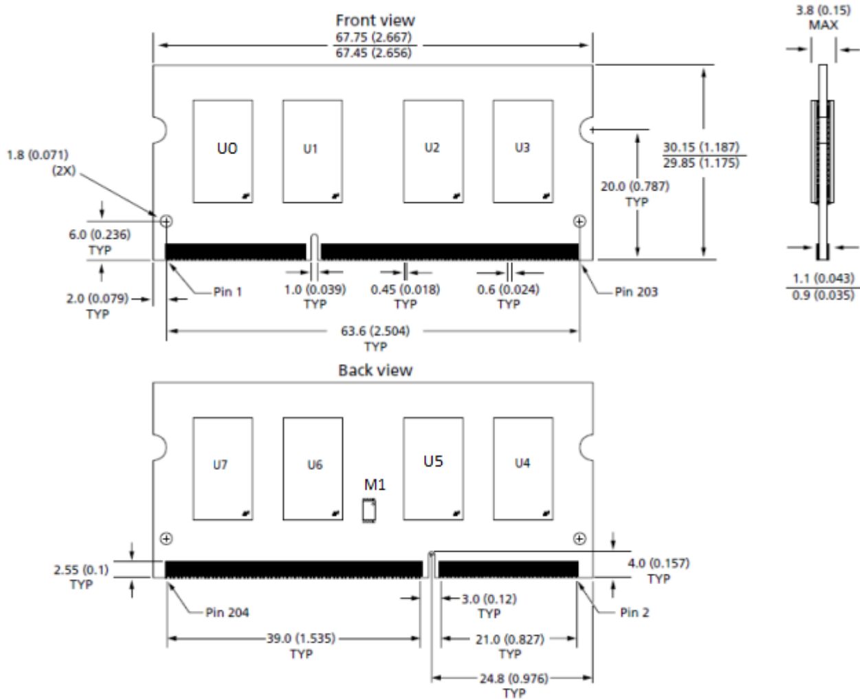
Figure 1 - Package Dimensions_ HXMSH4GS03A2F1CL16KI
