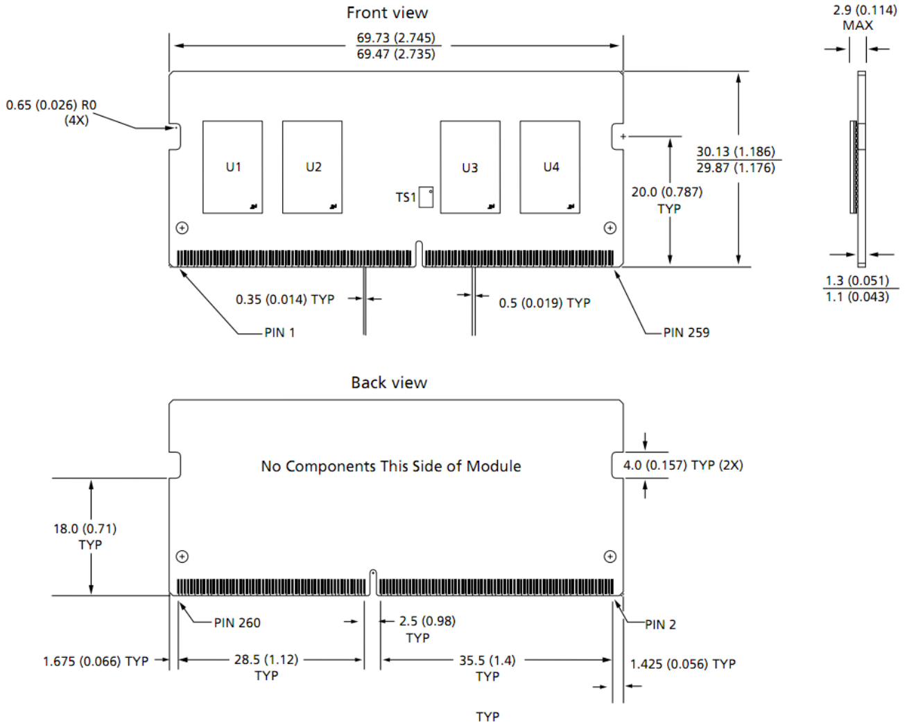
Figure 2 - Package Dimensions_SCC04GS04H3F1C-32AA
