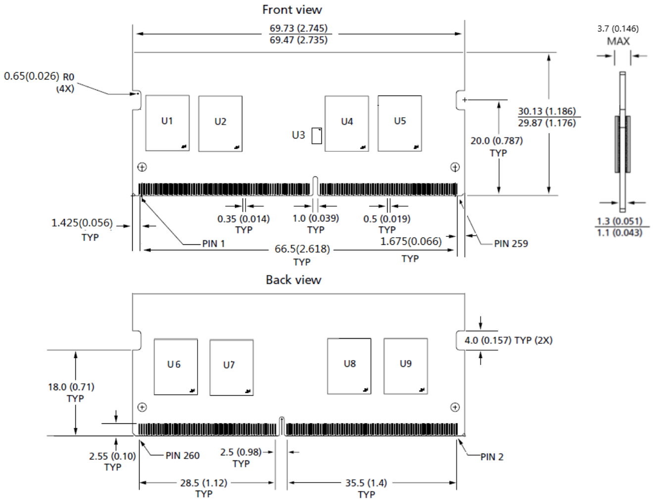
Figure 2 - Package Dimensions_SCC08GS03C2F1C-32AA
