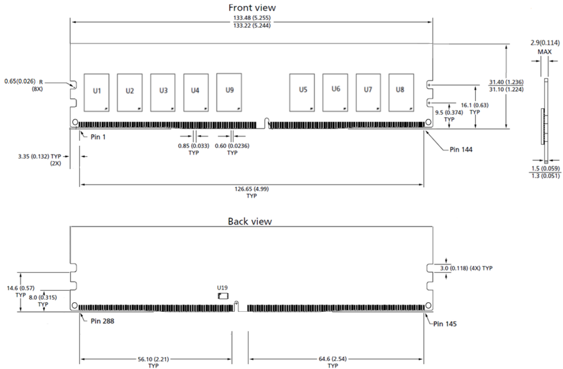
Figure 3 – Package Dimensions_SCC16GE03H4F1C-32AA
